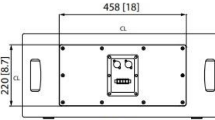
REAR
