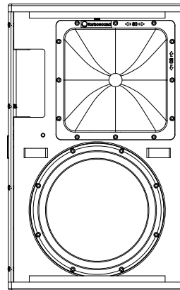
FRONT (Grille removed for clarity)
